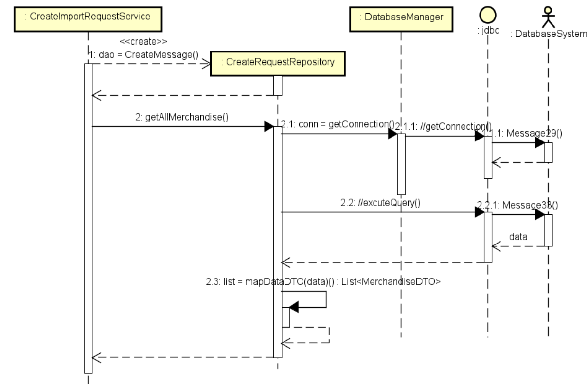
Interaction Ref: refFetchMerchandiseInfo
